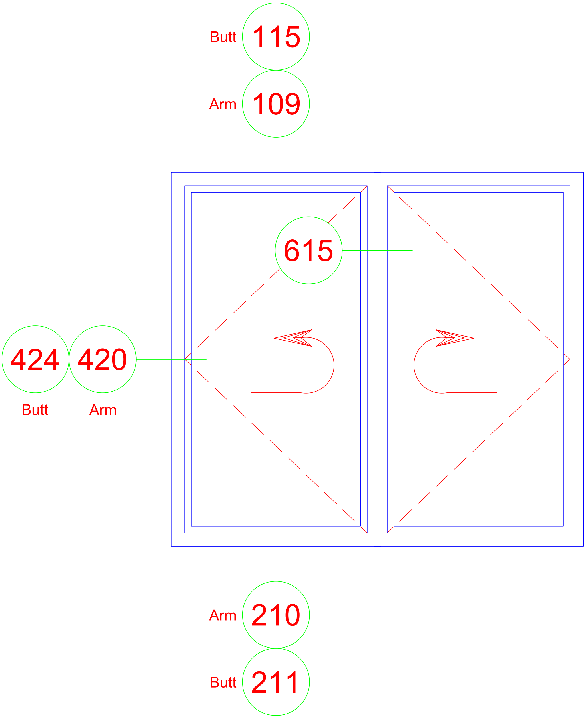
2700 Inside Glazed Casement In | Casement In (Meeting Rail = M.R.) Left Swing | Right Swing 4-bar Arms (Butt Hinges) Cam Locks
